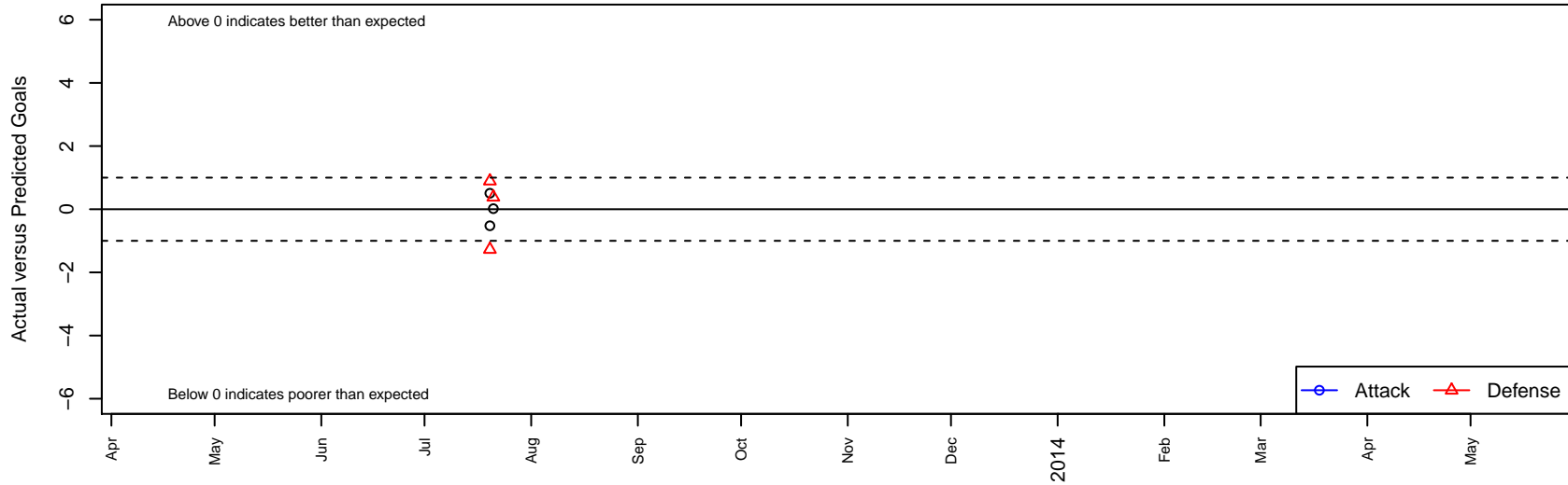
RSF Attack B94 Dots are actual minus expected GF (blue circles) and GA (red triangles). Blue line is smoothed change in attack strength. Red is smoothed change in defense strength.
